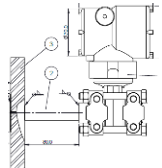
Schematic of a direct mount
