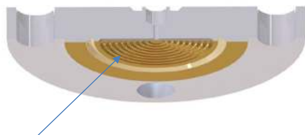
Example of a blind flange cut through to understand diaphragm thickness and diaphragm seal chamber for minimal filling fluid, tailored to the application and specifications. Both pictures relate to gold coating on diaphragm and seal.
