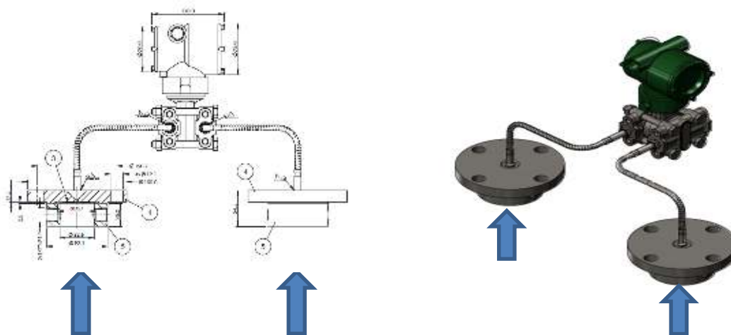
An example of a delta-P measurement (note the same length capillaries)
