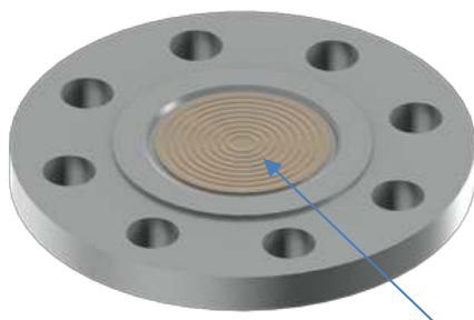
Example of a blind flange seal with the diaphragm welded to the flange. Diaphragm has special convolution to transmit the pressure and has a thickness of 75-150 micron.
